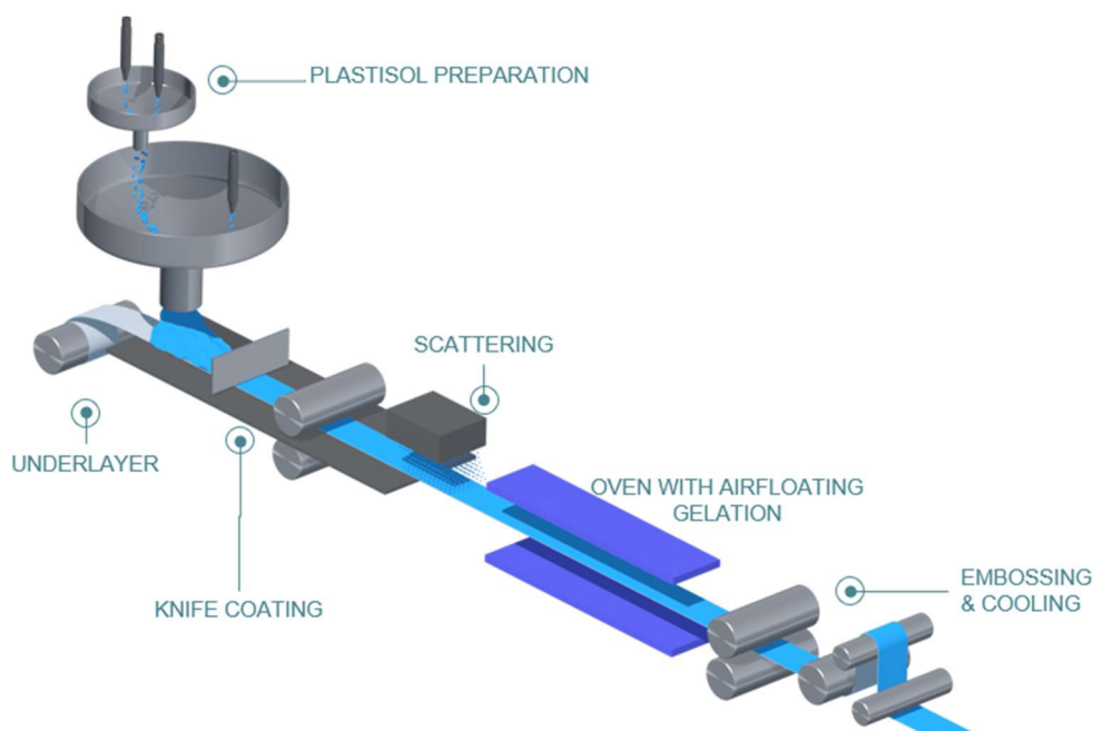
Figure 3: Coating process
